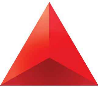
TETRAHEDRON (FIRE)
