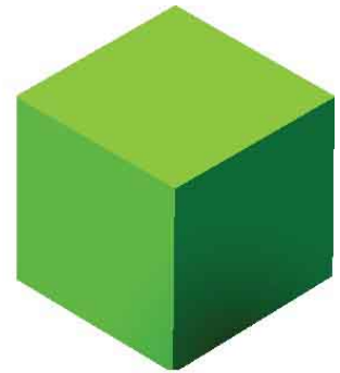
CUBE (EARTH)
