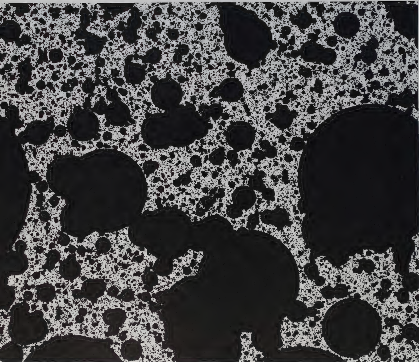
Plates 308 and 309 □ LARGER ROUND TREMAS, IN BLACK, AND RANDOM FORKED WHITE THREADS (DIMENSIONS D=1.7500 AND D=1.5000 )
