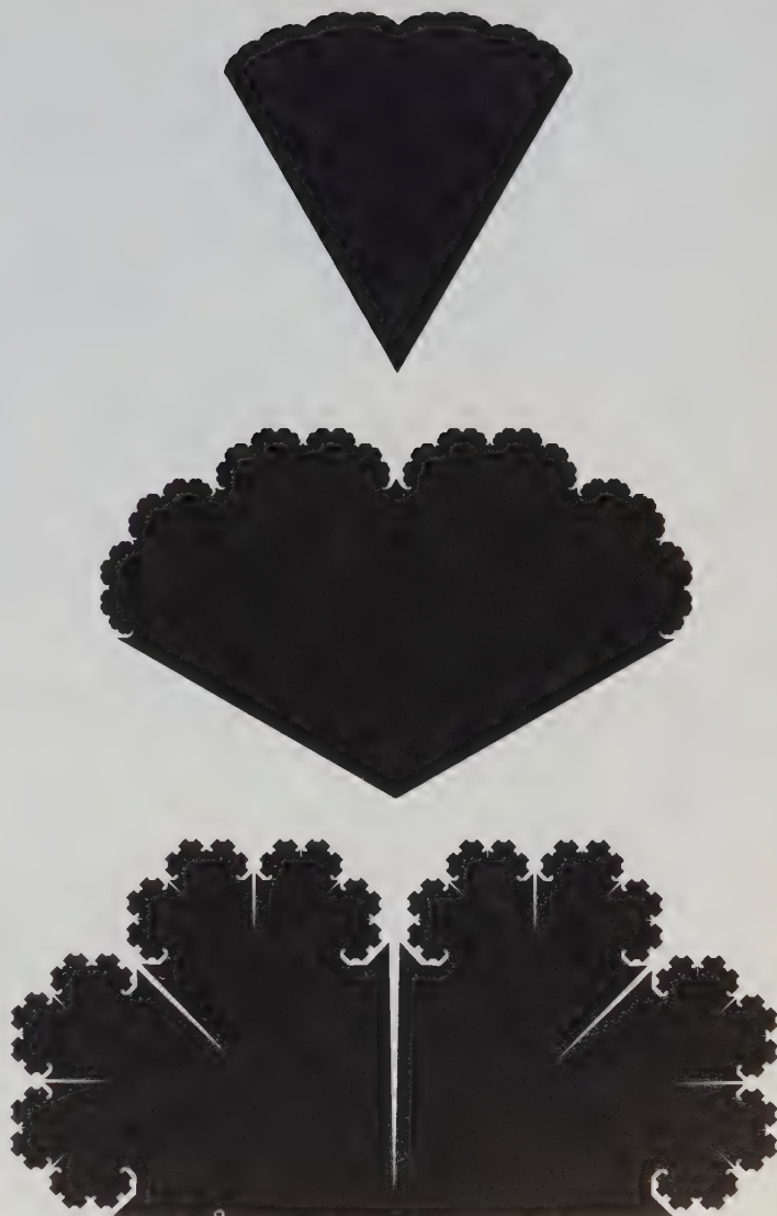
Plate 163 ■ FLATTENED FRACTAL MODELS OF PLANT FLOWERS
